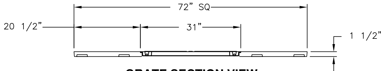
GRATE SECTION VIEW
