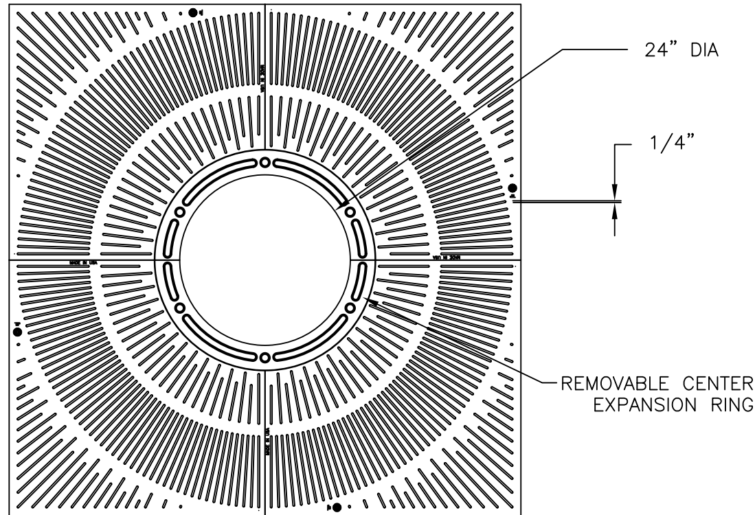
GRATE PLAN VIEW
